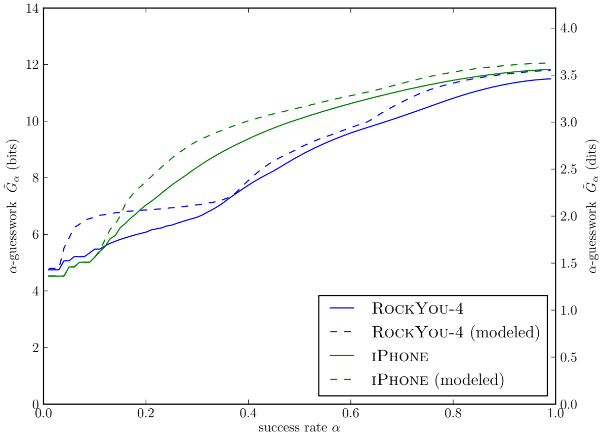
Figure 4.1: Guessing curves for the 4-digit sequences found in RockYou passwords and iPhone unlock codes, as well as the best-fit model distributions produced by linear regression on 25 variables (see Table 4.2).
